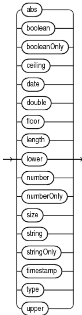
Figure B-8 json_item_method
